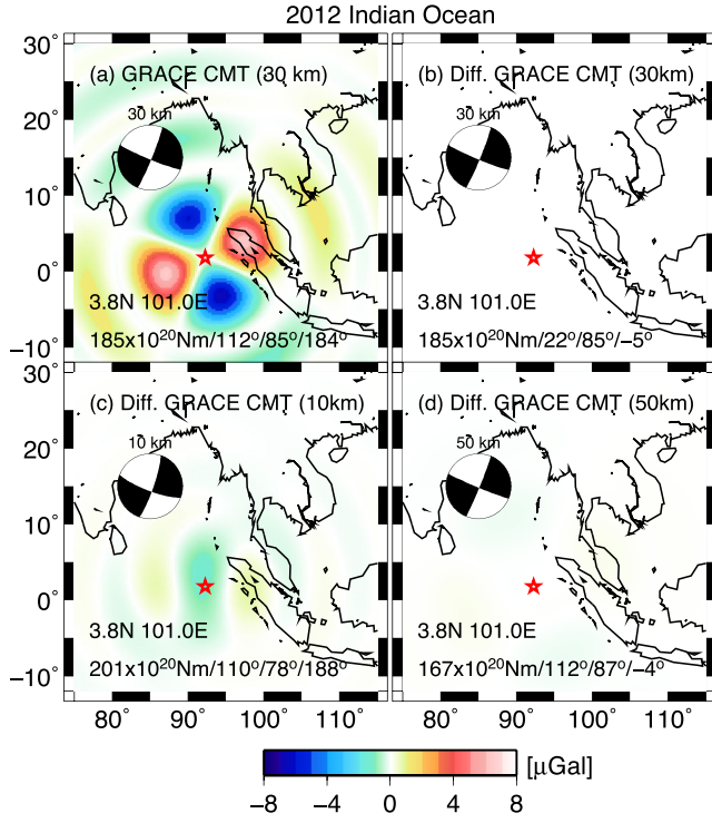
Figure 29. Same as Figure 12 for the 2012 Indian Ocean earthquake. The location of the centroid is 3.8^\circ\text{N} and 101.0^\circ\text{E} . Figure 29a stands for the WNW-ESE fault plane while Figure 29b the NNE-SSW plane at the same depth of 30 km. Note that the surface gravity is not significantly different even with a wide range of variation in centroid depth.
