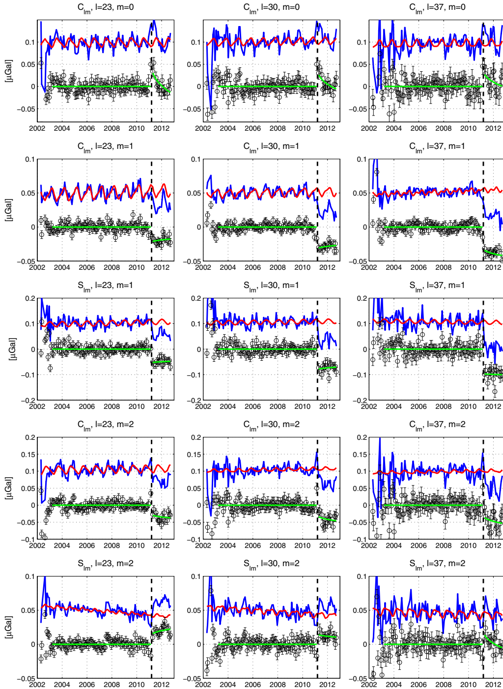
Figure 20. Same as Figure 7 for the 2011 Tohoku-Oki (Japan) earthquake. The GRACE coefficients were rotated in the coordinate system where the z axis locates at 38.5^{\circ}\text{N} and 142.6^{\circ}\text{E} . Higher noise in 2002 is due to the use of RL04 GRACE products. The quality of the product is improved with RL05 as shown in the rest of the years.
