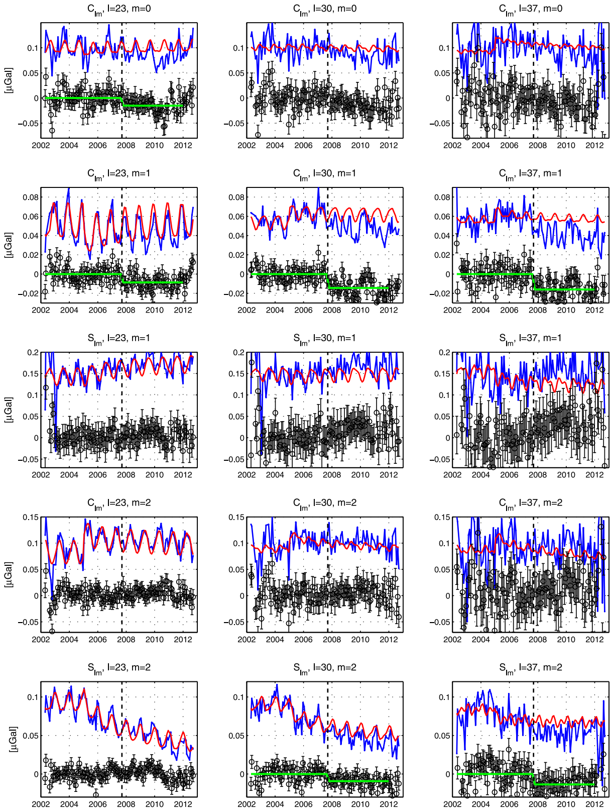
Figure 14. Same as Figure 7 for the 2007 Bengkulu earthquake. Note that the C_{l,1} coefficients present a significant step before and after the epoch of the event in 2007. This particular earthquake was strongest in the component of M_{r,\theta} .
