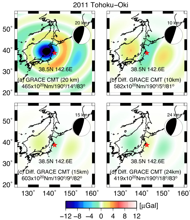
Figure 24. Same as Figure 12 for the 2011 Tohoku-Oki (Japan) earthquake. The location of the centroid is 38.5^{\circ}\text{N} and 142.6^{\circ}\text{E} .
