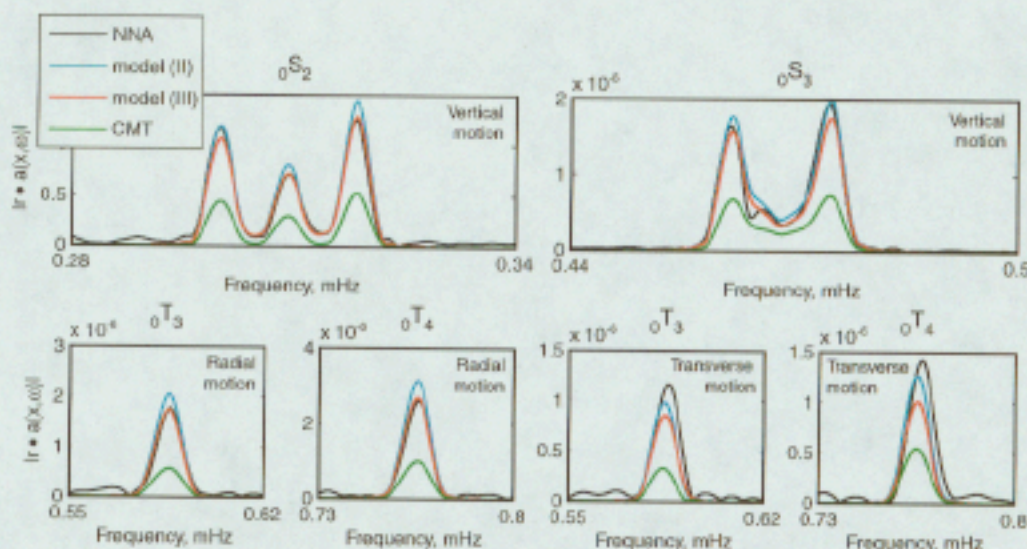
Fig. 7. Comparison of data (NNA, at Nana, Peru) and synthetics from various models. Low-order spheroidal modes {}_0S_2 , {}_0S_3 at vertical component and toroidal modes {}_0T_3 , {}_0T_4 at horizontal component are shown (top). A Hann taper is applied to 144-hour time series of vertical motion before discrete Fourier transformation. Similar tapering was performed on 44-hour time series of radial and transverse horizontal motion before discrete Fourier transformation.
