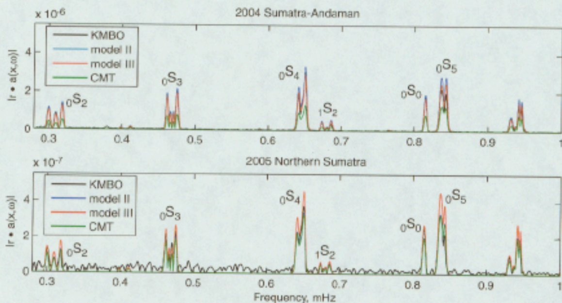
Fig. 8. Spectrum comparison for the 26 December 2004 Sumatra-Andaman and 28 March 2005 Northern Sumatra earthquakes using 127-hour records of vertical motion recorded at station KMBO (Kilima Mbogo, Kenya). Spectral predictions of the Harvard CMT solutions are graphed as well as spectra predicted from finite-rupture models from (4). Note the greater success of the CMT solution for the 2005 event, consistent with a smaller less complex rupture process.
