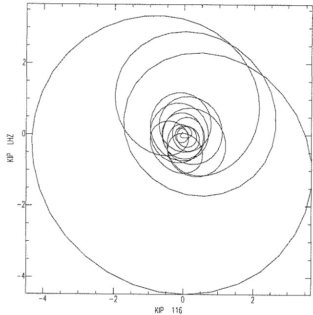
Figure 5. Rayleigh-wave particle motion in the 'sagittal' plane, reconstructed by plotting the vertical component of motion against the radial component ( AZM=116^\circ ). A clear retrograde ellipse is evident, but the semi-major axis is tilted away from the vertical by the effects of anisotropy.
