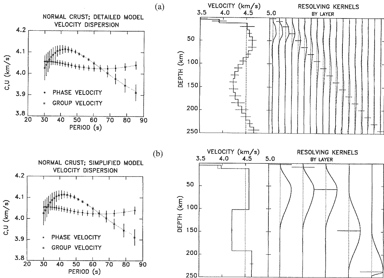
Figure 10. (a) Summary of detailed shear-velocity model for Hawaiian Swell with normal-thickness crust. Left. Open squares represent group velocities; filled circles represent phase velocities; error bars are one standard error; dashed lines are inverse fits to observations. Right. In the velocity model the dashed line represents the starting values and the solid line represents the final values. Resolving kernels are normalized to the maximum value, and show that \beta_V is reasonably well resolved to depths of z \sim 150 km. (b) As (a), but for the simplified shear-velocity model. Here \beta_V is reasonably well resolved at all depths.
