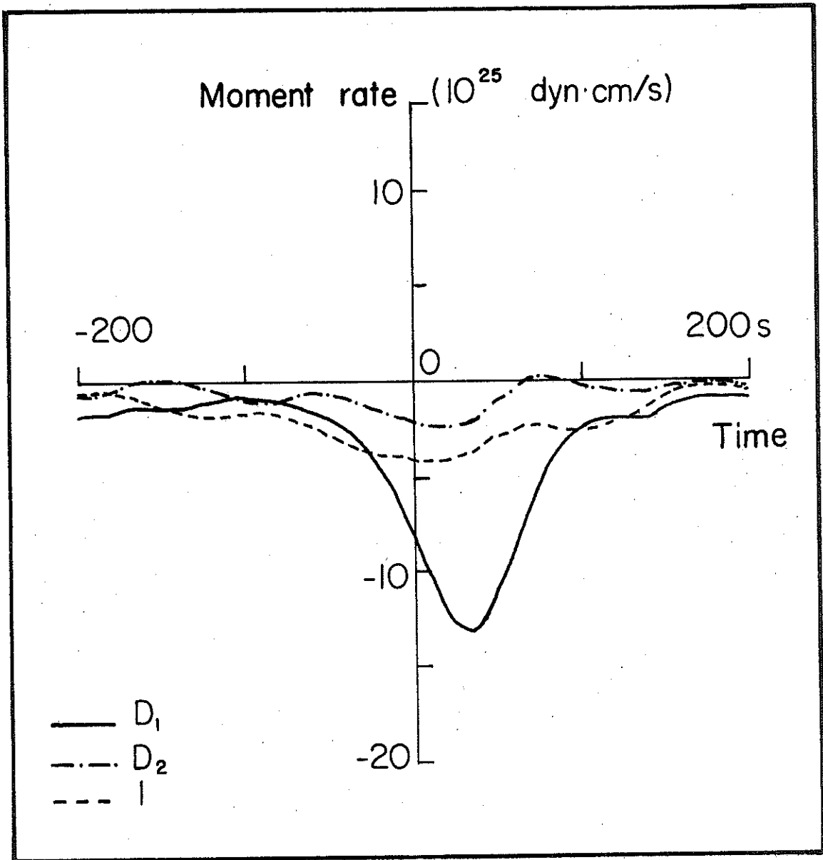
Figure 2.8. Moment rate function of both deviatoric ( D_1, D_2 ) and of the isotropic (I) moment rate tensor components obtained by Gilbert and Dziewonski. Details of the geometry are listed in Table 2.2. D_1 is essentially equivalent to the double-couple sources of Mendiguren and Furumoto and Fukao.
