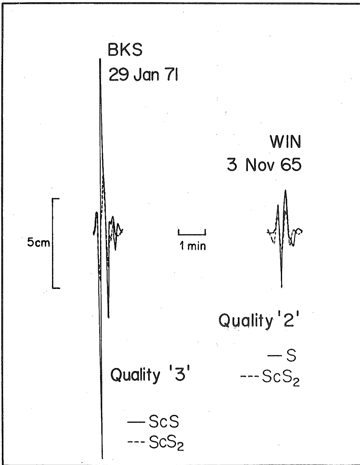
Figure 1.3. Samples of 'Quality 3' and 'Quality 2' pairs of cross-correlated phases. Distances are 59.6^\circ for Berkeley (BKS) and 85.2^\circ for Windhoek (WIN).
