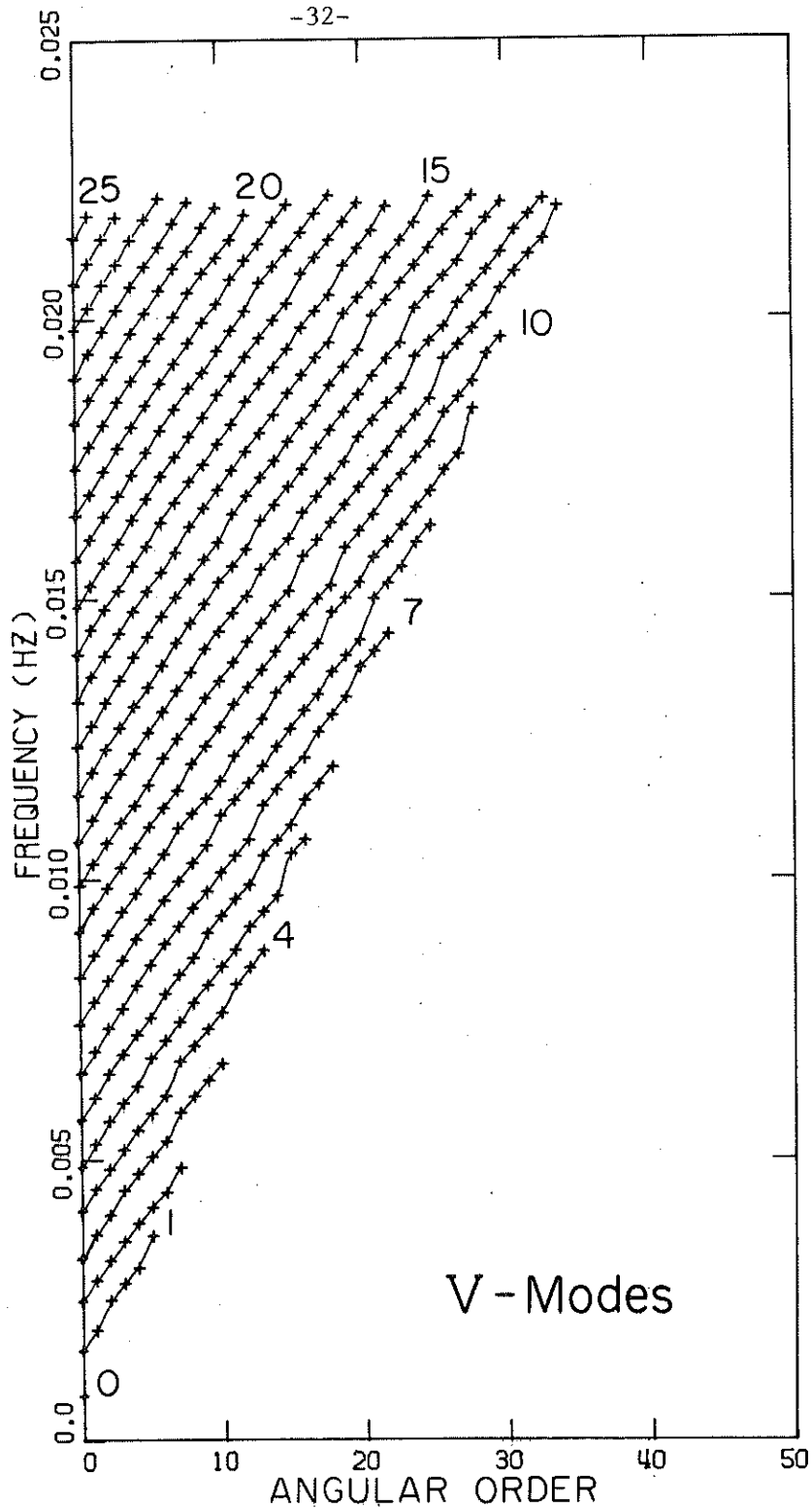
Figure 1.5. Frequency versus angular order plot of the V family of modes. Pseudo-overtones are traced and labeled according to the new proposed nomenclature. Note the easy integration of the radial modes into the family.
