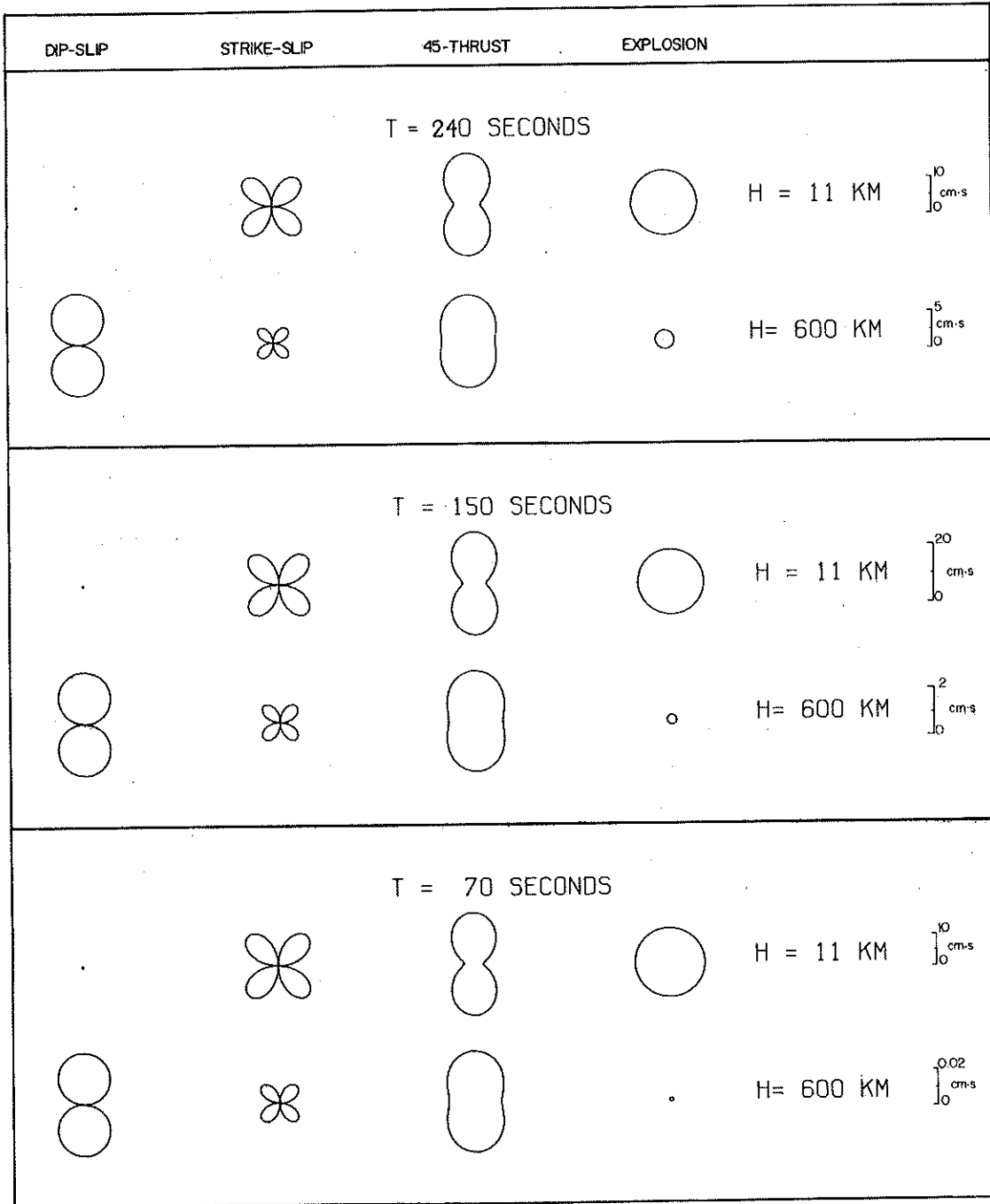
Figure 2.2. Radiation patterns of Rayleigh waves for both a surface event and a deep earthquake are compared for various source geometries at three different periods. The station distance is \lambda=60^\circ and a common moment rate of 10^{27} dyn.cm/s is assumed. The different scales are common to the four figures on a given line, but vary from line to line.
