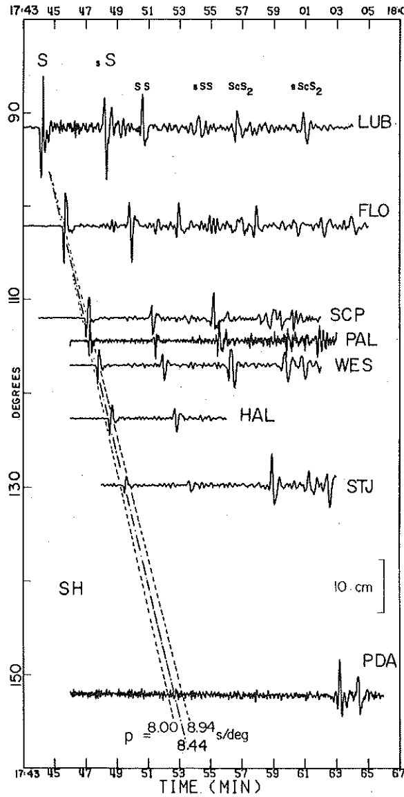
Figure 3.4. Observed data profile for event 1. The seismograms have been equalized to a standard magnification of 1500, and rotated into SH polarization. The oblique lines show the result of alignment of the sharp onsets with a straight edge ( p_0 = 8.44 s/deg), and lines of constant slowness corresponding to velocities of 6.8 and 7.6 km/s at the core-mantle boundary.
