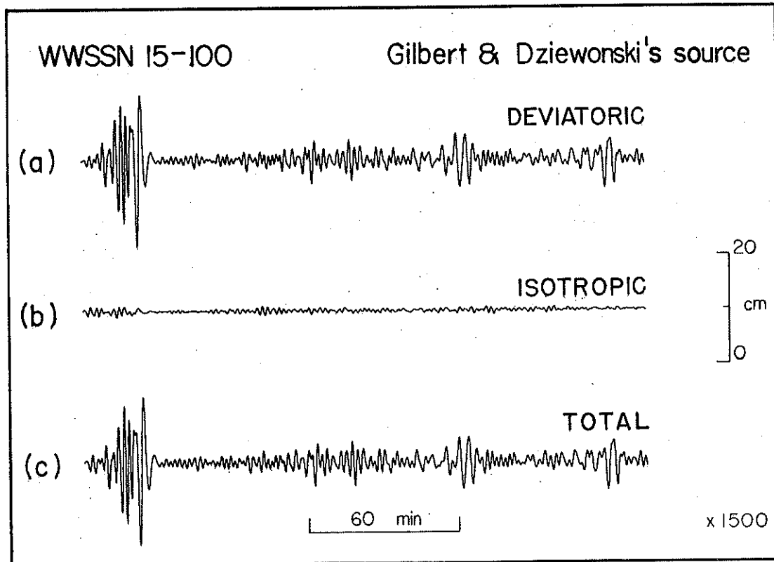
Figure 2.13. Synthetic seismograms obtained for Gilbert and Dziewonski's source, assuming a WWSSN instrument. (a) Deviatoric sources D_1 and D_2 only. (b) Isotropic source (I) only. (c) Full source. This type of record was used in Gilbert and Dziewonski's inversion. The geometry of the station is that of Pasadena.
