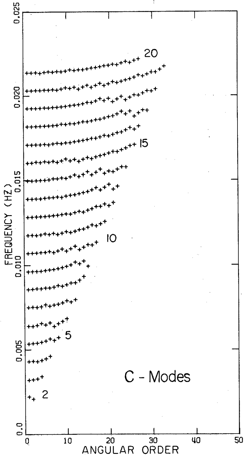
Figure 1.6. Frequency versus angular order plot of the C family of modes. Pseudo-overtone numbers are labeled according to the new proposed nomenclature.
