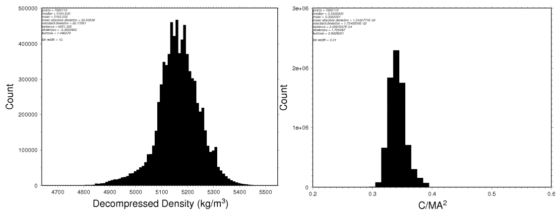
[Fig.: Some statistics for a sample suite (#230607) of Mercurian models.]
