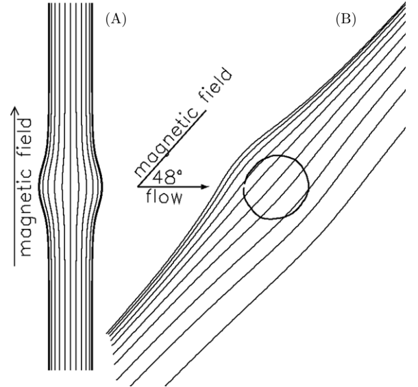
Figure 2. Draped interstellar magnetic field lines: (a) in Parker's solution (star at rest relative to the interstellar medium with insignificant plasma density), and (b) obtained from 3D MHD simulations for spherically symmetric solar wind and interstellar magnetic field of 20\mu\text{G} , inclined 48^\circ to interstellar plasma flow (projection on a plane containing interstellar flow and field vectors).
