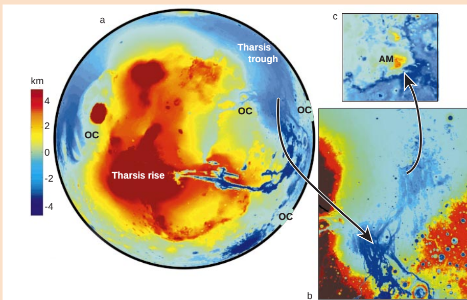
Figure 3 Topography 98 of Tharsis rise and Tharsis trough 28 . a , Topography, which has been saturated at \pm 5 km, with pole-to-pole slope 98 removed. Image is centred on 260° E longitude and view is from 10° north of equator. Outflow channel locations are marked by 'OC'. b , Channel detail in Chryse and Acidalia Planitiae (0°–60° N, 300°–0° E, Mercator projection; elevation range is –3.9 km to 0 km). c , The inlier Acidalia Mensa ('AM'), whose southern and eastern boundaries are channels (Mercator projection; elevation range is –3.0 km to –1.5 km). Eastern channel extends northwards of 50° N.
