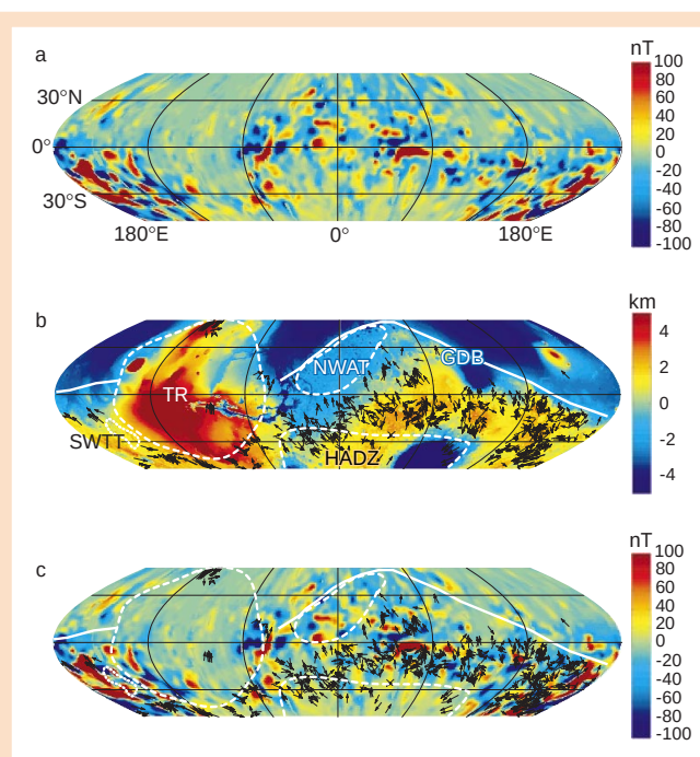
Figure 4 Comparison of martian magnetic field, topography and valley network locations. a , Radial component of the martian magnetic field at an altitude of 200 km (after ref. 106). Values saturated at \pm 100 nanotesla (nT). Sinusoidal projection to \pm 47.5^\circ latitude. b , Topographic map of Mars (after ref. 98), saturated at \pm 5 km elevation, and locations of valley network systems 13 . Database is limited to latitudes less than \pm 47.5^\circ , which is the approximate limit of valley network distribution. Features indicated are the Tharsis rise (TR), global dichotomy boundary (GDB), northwestern Arabia Terra (NWAT), southwestern Tharsis trough (SWTT) and Hellas-Argyre disruption zone (HADZ). TR, NWAT, SWTT and the area north of GDB are regions of valley network exclusion by erosion and/or deposition and cannot be judged for the level of correlation of valley networks with anomalies in the remanent magnetic field. Likewise, TR, HADZ and the area north of GDB are regions of magnetic field exclusion by the presence of post-main-field crustal ages or crustal disruption 34 . c , Valley networks and features in b superposed on magnetic anomaly map.
