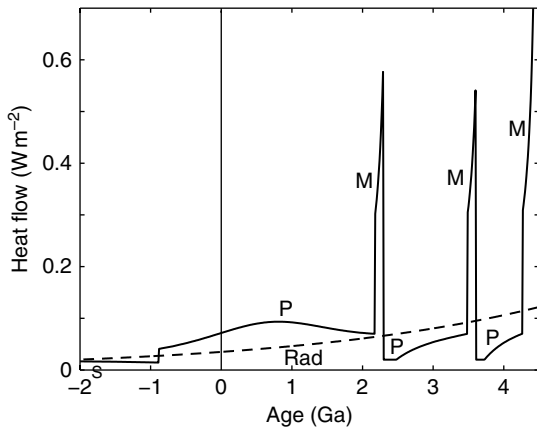
Figure 2 Computed heat flow as a function of age for the nonmonotonic model (dark line) and the radioactive heat generation as heat flow (thin dashed line). The modes of convection are (M) mush ocean, (P) plates, and (S) stagnant lid. The model resolves the expected duration of episodes, but no attempt was made to fine-tune the timing of transitions.
