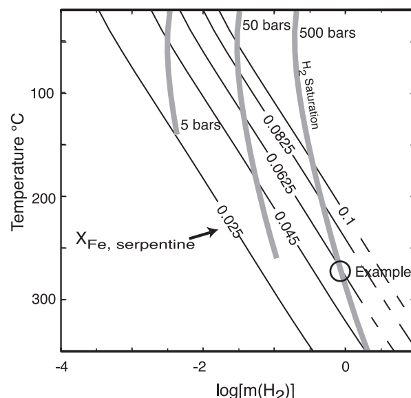
Fig. 2. Phase diagram as in Fig. 1 showing isopleths of SBM buffer equilibria for serpentinites with X_{Fe} in crysotile ranging from 0.1 to 0.025. H_2 partial pressure contours are thick gray lines.
