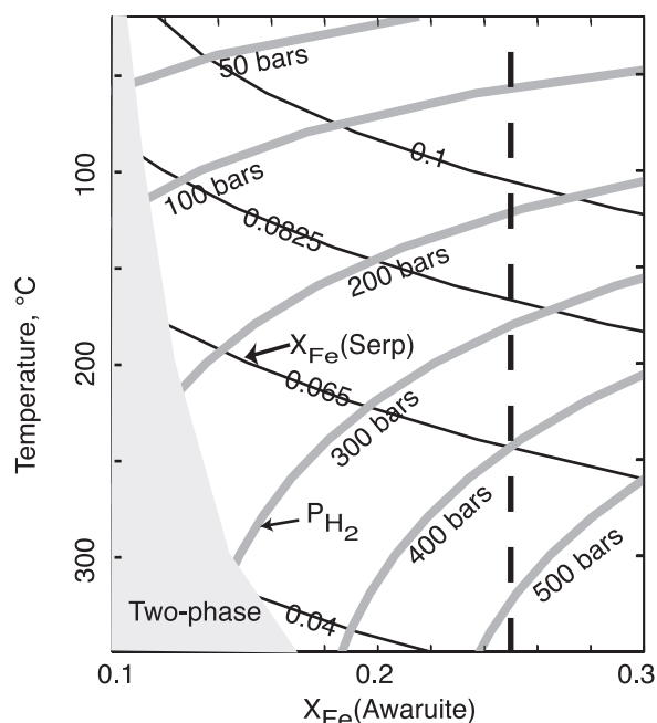
Fig. 3. Hydrogen partial pressures and X_{Fe} in serpentine in equilibrium with brucite, magnetite, and awaruite as a function of X_{Fe} in awaruite and temperature. The two-phase region (awaruite plus Ni solid solution) is shaded.
