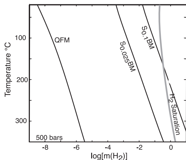
Fig. 1. Molality of H_{2(aq)} for SBM buffer (reaction 3) as a function of temperature at 500 bars total fluid pressure. Isopleth S_{0.1}BM represents high-Fe serpentinite, with X_{Fe} = 0.1 in crysotile and X_{Fe} = 0.07 in brucite, and S_{0.025}BM represents low-Fe serpentinite, with X_{Fe} = 0.025 in crysotile and 0.0175 in brucite. QFM buffer and hydrogen solubility bars are shown.
