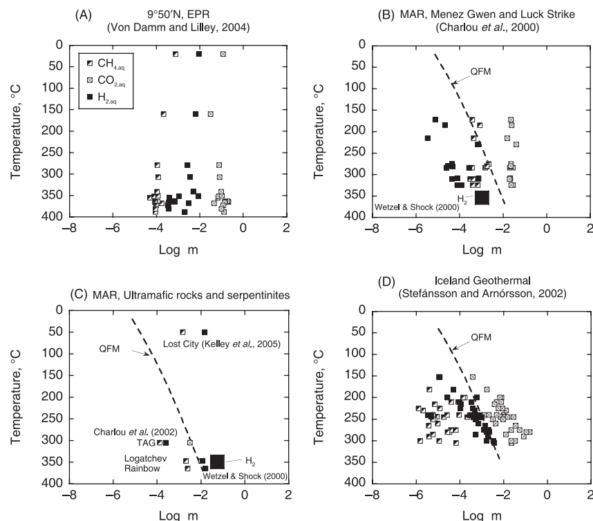
Fig. 3 Molal concentrations of aqueous \text{CH}_4 , \text{CO}_2 and \text{H}_2 from (A) basalt-hosted vents and diffuse flow from 9°50'N East Pacific Rise (Von Damm & Lilley, 2004), (B) basalt-hosted vents from the Mid-Atlantic Ridge (Menez Gwen and Lucky Strike; Charlou et al. , 2000), (C) vents from ultramafic rocks and serpentinites of the Mid-Atlantic Ridge (TAG, Logatchev, Rainbow; Charlou et al. , 2002) and Lost City (Kelley et al. , 2005), and (D) geothermal drill holes in active geothermal systems in Iceland (Stefánsson & Arnórsson, 2002). Theoretical calculations of \text{H}_{2,\text{aq}} concentrations of hydrothermal fluids in basalt-hosted and ultramafic submarine hydrothermal systems are shown by the large solid square in diagrams B and C, respectively (Wetzel & Shock, 2000).
