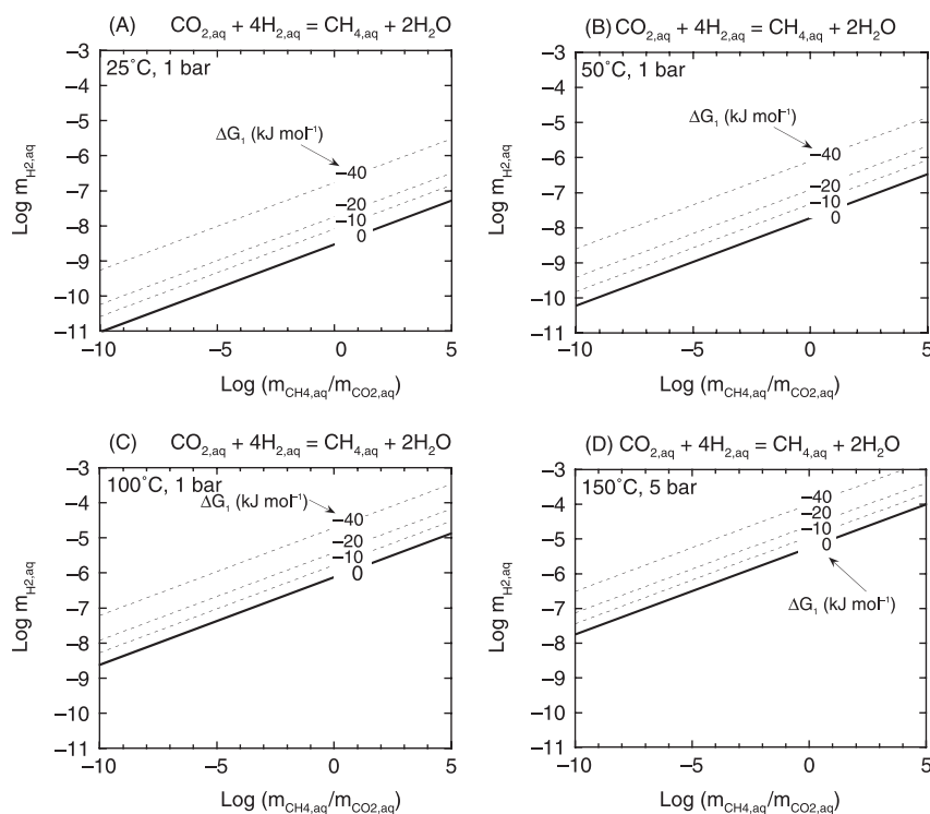
Fig. 2 Dependence of the concentration of aqueous H_2 on the molal ratio of CH_4 to CO_2 and the Gibbs energy for the methanogenic reaction 1 at 25, 50 100 and 150 °C and low pressures. Solid line denotes equilibrium conditions and the dashed lines labeled -10 and -20 kJ mol ^{-1} denote limiting conditions for starvation and growth, respectively, for methanogens (cf. Hoehler, 2004; computed using SUPCRT, Johnson et al. , 1992).
