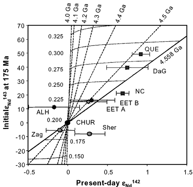
Fig. 2. \epsilon(^{143}\text{Nd}) versus \epsilon(^{142}\text{Nd}) . Condordia diagram for the ^{147}\text{Sm} - ^{143}\text{Nd} and ^{146}\text{Sm} - ^{142}\text{Nd} systems, after Borg et al. (2001). With the sole exception of Shergotty, the shergottites are consistent with derivation from reservoirs that differentiated from chondritic at \sim 4.51 Ga, in agreement with the Rb-Sr system. The nakhlite-Chassigny (NC) source (and perhaps the Shergotty source) is required to be derived from a reservoir that has undergone a more complex evolution. Abbreviations: Sher = Shergotty; Zag = Zagami; EET A and EET B = EET 79001A and EET 79001B; ALH = ALH 77005; QUE = QUE 94201; DaG = Dar al Gani 476; CHUR = Chondritic values at 175 Ma.
