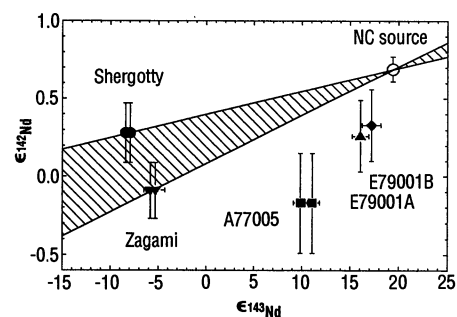
Fig. 3. Plot of \epsilon_{142}\text{Nd} data for the shergottite meteorites versus time-projected \epsilon_{143}\text{Nd} for these rocks when their parent melts crystallized at \sim 180 Ma. Mixing relations are linear in this plot. Mantle melts from the NC source assimilating a putative crustal component present in Shergotty and Zagami at 180 Ma are constrained to the cross-hatched area. Meteorites A77005 and E79001A and B do not plot within this zone and therefore are inconsistent with a two-component mixing model. The parental melts of the shergottites do not appear to have been derived from the NC source.
