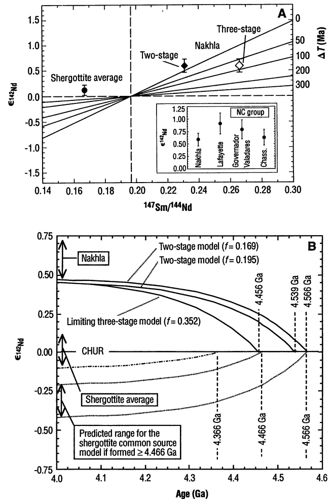
Fig. 2. (A) An \epsilon^{142}\text{Nd} isochron plot for the Nakhla source and the shergottite common source model. Individual data for the NC group meteorites are shown in the inset. The model age range for formation of the Nakhla source is obtained from tie lines connecting the data range to the CHUR reference point ( ^{147}\text{Sm}/^{144}\text{Nd} = 0.1967 ; \epsilon^{142}\text{Nd} = 0 ) and can be read off the \Delta T scale. The (preferred) two-stage model is for a single stage of fractionation with ^{147}\text{Sm}/^{144}\text{Nd} = 0.230 ( f_{\text{Sm}/\text{Nd}}^{146} = 0.169 ) obtained from a self-consistent two-stage model of \epsilon^{143}\text{Nd} evolution, as shown in the upper part of Fig. 1B (solid line). The limiting three-stage model is for the more complicated (extreme) model of \epsilon^{143}\text{Nd} evolution ( ^{147}\text{Sm}/^{144}\text{Nd} = 0.266 ; f_{\text{Sm}/\text{Nd}}^{146} = 0.352 ) shown by dashed lines in the upper part of Fig. 1B. (B) Time evolution plot for \epsilon^{143}\text{Nd} with fractionated mantle reservoirs indicated by curved evolution paths diverging from CHUR at their time of formation. The lowest age possible for differentiation of the Nakhla source is 4.539 Ga in the preferred two-stage model ( f_{\text{Sm}/\text{Nd}}^{146} \leq 0.195 ). In the extreme case of the three-stage model ( f_{\text{Sm}/\text{Nd}}^{146} \leq 0.352 , see Fig. 1B), a source formation age as low as 4.456 Ga is allowed. Evolution paths for a source with f_{\text{Sm}/\text{Nd}}^{146} = -0.151 are shown as dashed curves in the lower half of (B) for formation times of \Delta T = 0 and 100 Ma, and as a dot-dash curve for \Delta T = 200 Ma. If the shergottites were derived from a common source 1.3 Ga ago (Fig. 1A, solid lines), then this source must have been derived from a domain that either involved planetary recycling or remained unfractionated in the martian mantle for at least the first 200 million years of solar system history (dot-dash curve). It cannot have formed contemporaneously with the Nakhla source with Sm/Nd as fractionated as f_{\text{Sm}/\text{Nd}}^{146} = -0.151 .
