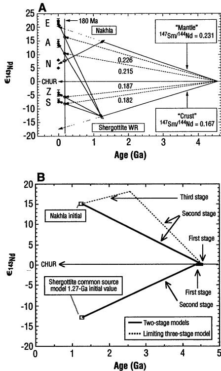
Fig. 1. (A) An \epsilon^{143}\text{Nd} time evolution plot for SNC meteorites and their source reservoirs showing growth in parts-in- 10^4 deviation ( \epsilon -units) in ^{143}\text{Nd}/^{144}\text{Nd} relative to that of CHUR. A single stage of evolution for the Nakhla source (N) is shown by the uppermost solid line (labeled "mantle") connecting the Nakhla initial point to the horizontal CHUR line at 4.57 Ga. In the case of the shergottites, estimation of ^{147}\text{Sm}/^{144}\text{Nd} in source reservoirs is problematic because of the complex isotopic record in these meteorites. A "common source" interpretation (unbroken lines) is based on the apparent isochronous relation for the whole-rock (WR) shergottites, shown by the convergence of their evolution paths for Shergotty (S), Zagami (Z), ALHA 77005 (A), and EETA 79001 (E) at 1.3 billion years. An alternate "multiple source" interpretation (broken lines) follows evidence for an \sim 180 -Ma crystallization age for the shergottites. A range of initial \epsilon^{143}\text{Nd} values is given by intersections of WR evolution paths with the vertical line at 180 Ma. Single-stage evolution paths for these sources are drawn for the interval 180 Ma to 4.57 Ga. (Marked values are ^{147}\text{Sm}/^{144}\text{Nd} ratios.) (B) Schematic of possible reservoir formation and evolution histories subject to constraints from ^{142}\text{Nd}/^{144}\text{Nd} . Two possible evolution paths for two- and three-stage models of the Nakhla source are shown in the positive \epsilon^{143}\text{Nd} field. The (limiting) three-stage model has been selected to have a second-stage fractionation factor of 2 times that of the two-stage model.
