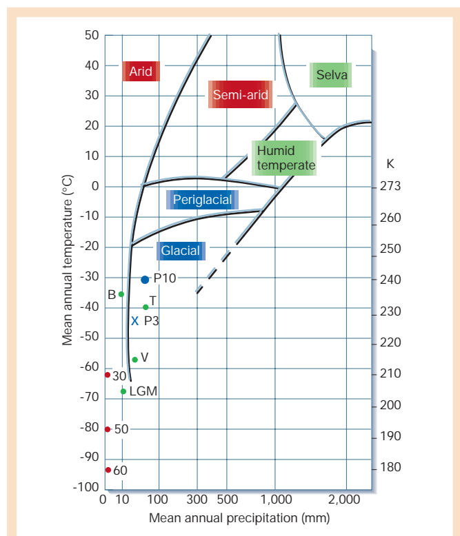
Figure 7 Morphogenetic regions for climate-related landforms on Earth 91 . Note the expanded precipitation scale at lower values. Modern terrestrial glacial environments include Taylor Dome (T) and Vostok (V) in Antarctica. Beacon Valley (B) occurs in the cold-arid, nonglaciated Dry Valley region of Antarctica. Conditions inferred from the last glacial maximum (LGM) in Antarctica were most similar to those of modern middle latitudes on Mars (30, 50 and 60 are the Mars conditions at the indicated latitudes). Modelled conditions 118 for ancient Mars at 300 mbar (300 hPa) atmospheric pressure (P3) and 1,000 mbar (P10) could have been comparable to the cold glacial conditions on modern Earth.
